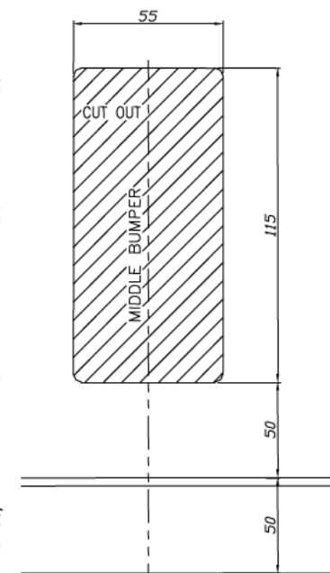
UNDERSIDE BUMPER
